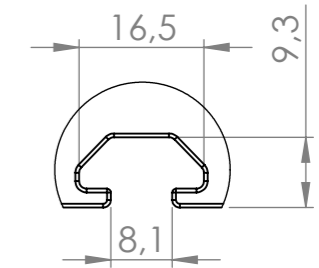
DETAIL B - Type 30 T-slot
