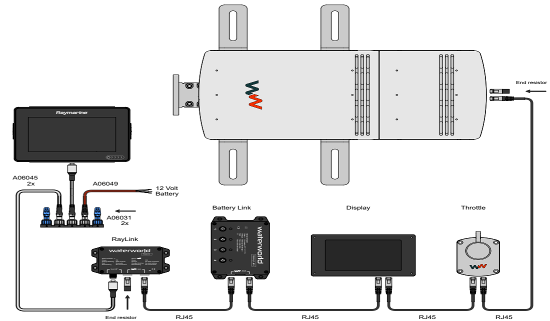
Connection diagram RayLink
